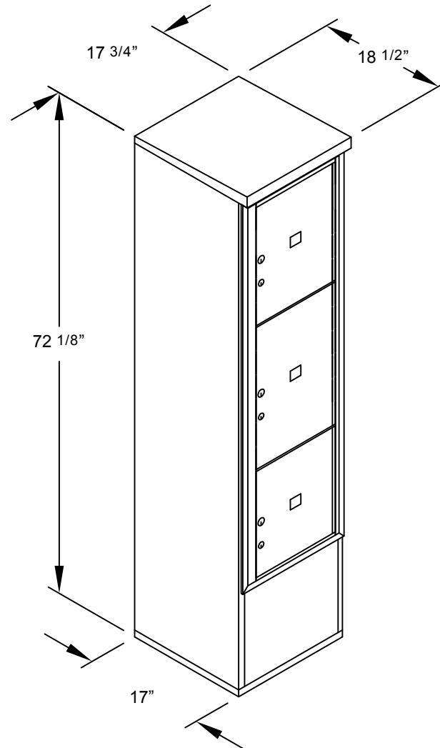
MODEL #3916S-3P - FRONT LOADING
