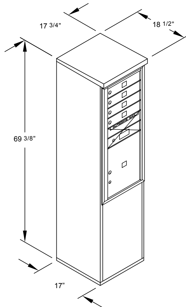
MODEL #3911S-04 – FRONT LOADING
