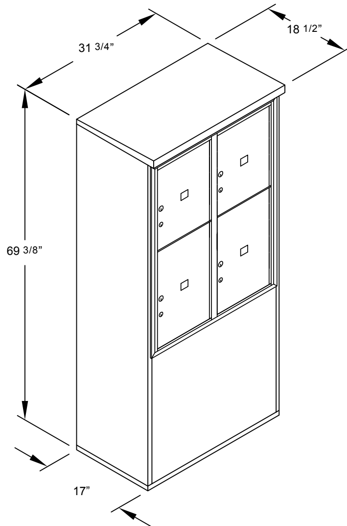
MODEL #3911D-4P - FRONT LOADING
