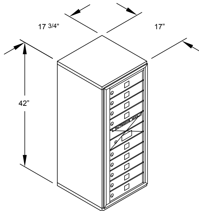
MODEL #3811S-09 – FRONT LOADING
