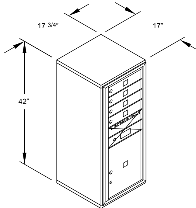
MODEL #3811S-04 - FRONT LOADING
