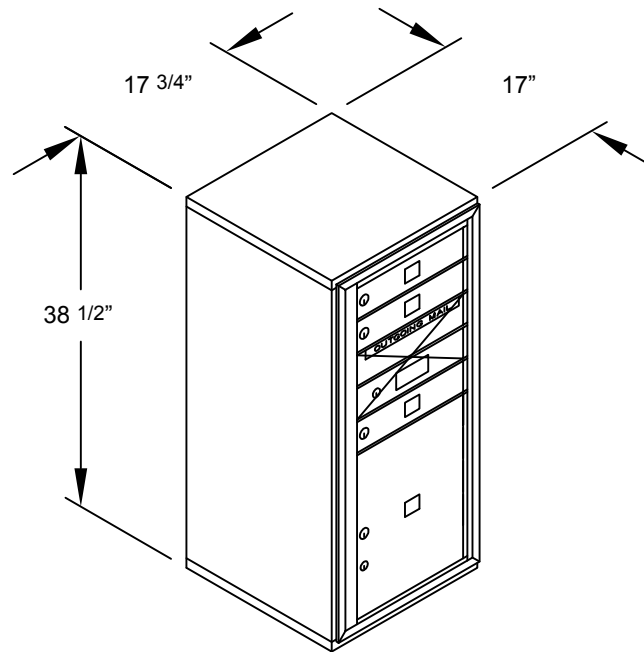
MODEL #3810S-03 - FRONT LOADING
