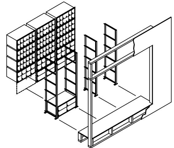
2212-COMBO REAR LOADING (12) '#1' DOORS WITH COMBINATION LOCKS
