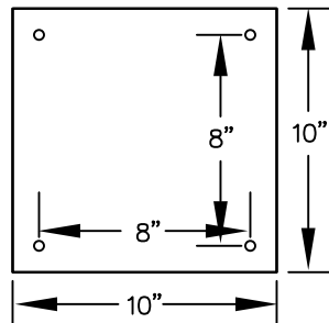
BASE BOLT PATTERN
