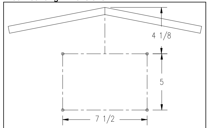
4750 Mounting Dimensions
