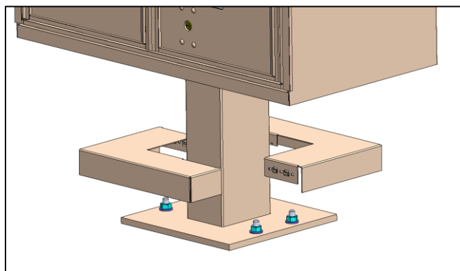
Figure 2: Pedestal Cover before Installation
