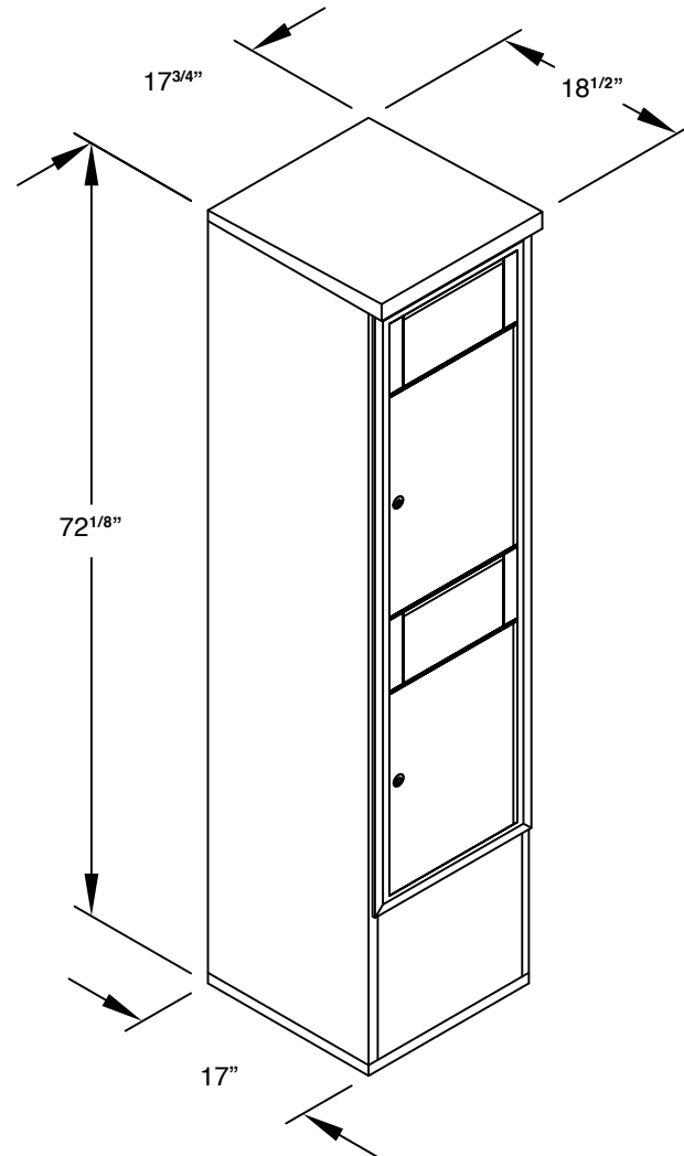
MODEL #3916S-2B - FRONT LOADING
