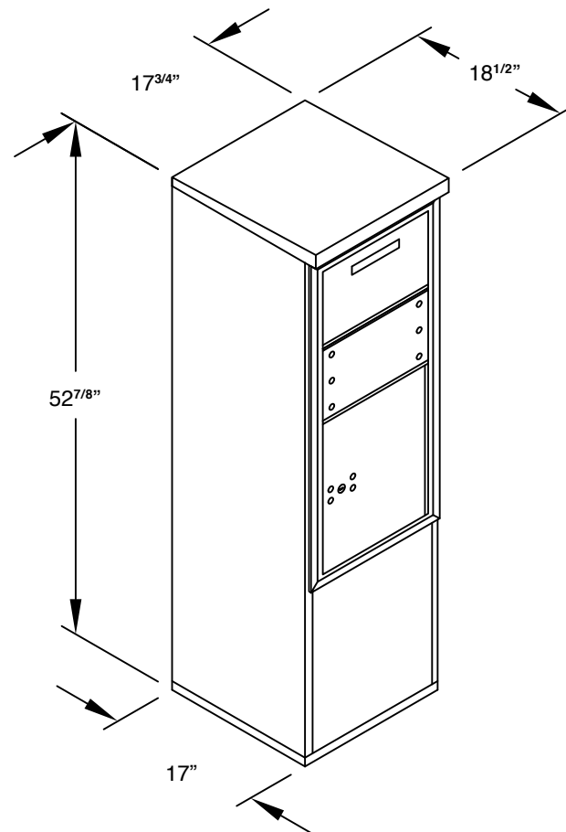
MODEL #3910S-1C - FRONT LOADING
