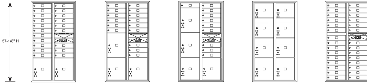
3716D-20 (20 MB1, 2 PL4.5, OM2) 3716D-15 (15 MB1, 2 PL4.5, 1 PL5, OM2) 3716D-10 (10 MB1, 2 PL4.5, 2 PL5, OM2) 3716D-8P (2 PL3, 4 PL4, 2 PL4.5) 3716D-29 1 (29 MB1, OM1.5)
