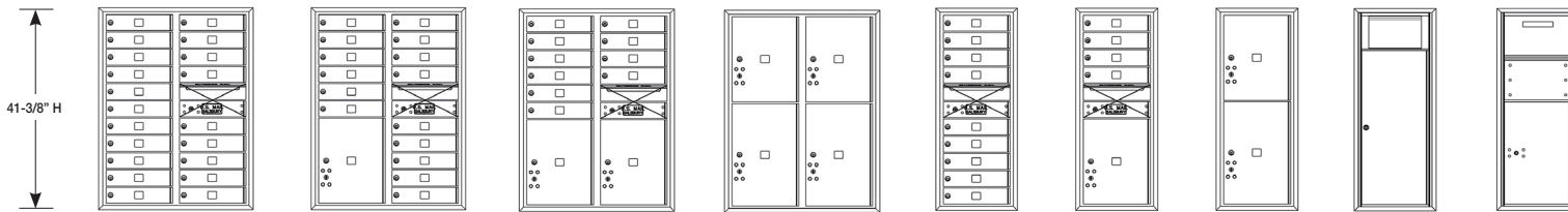
3711D-20 (20 MB1, OM2) 3711D-15 (15 MB1, 1 PL5, OM2) 3711D-10 (10 MB1, 2 PL5, OM2) 3711D-4P (2 PL5, 2 PL6) 3711S-09 (9 MB1, OM2) 3711S-04 (4 MB1, 1 PL5, OM2) 3711S-2P (1 PL5, 1 PL6) 3711S-1B 1 (1 Receptacle Bin) 3711S-1C 1 (1 Collection Box)
