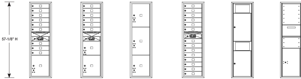
3716S-09 (9 MB1, 1 PL4.5, OM2) 3716S-06 (6 MB1, 1 PL3, 1 PL4.5, OM2) 3716S-3P (1 PL4.5, 1 PL5, 1 PL6) 3716S-14 1 (14 MB1, OM1.5) 3716S-2B 1 (2 Receptacle Bins) 3716S-1C 1 (1 Collection Box)
