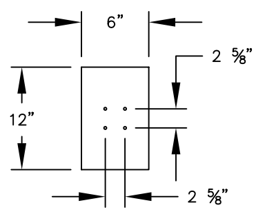
PEDESTAL TOP BOLT PATTERN
