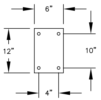
PEDESTAL BASE BOLT PATTERN
