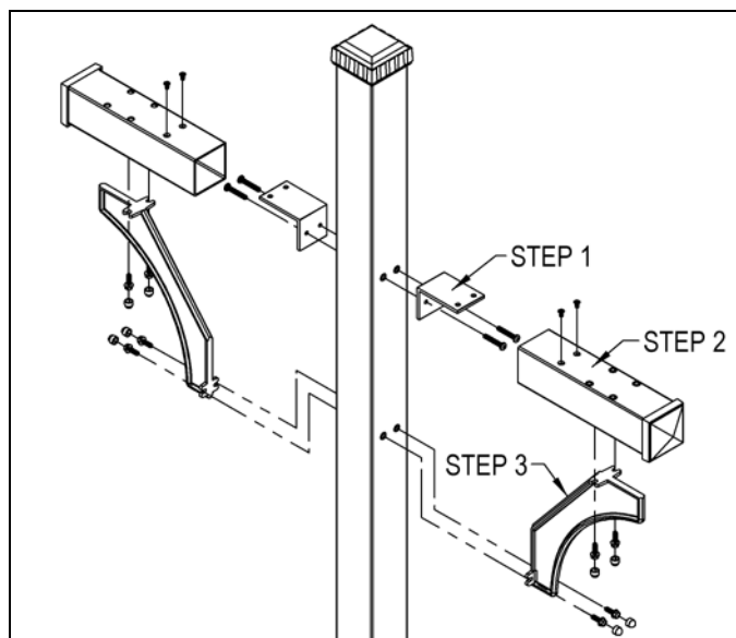
4872 and 4874 Assembly
