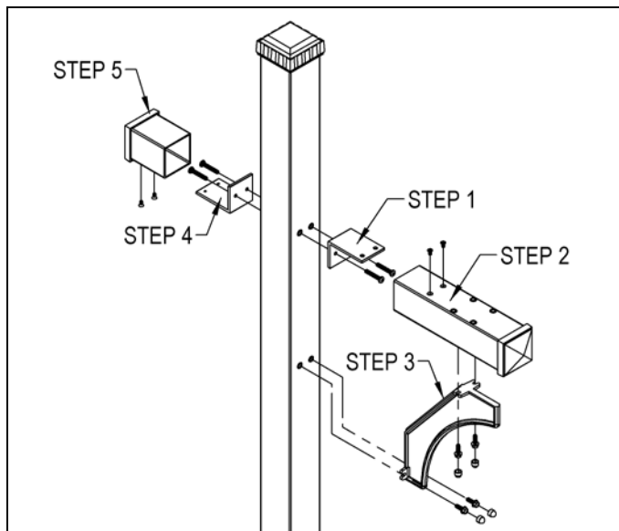
4870 Assembly
